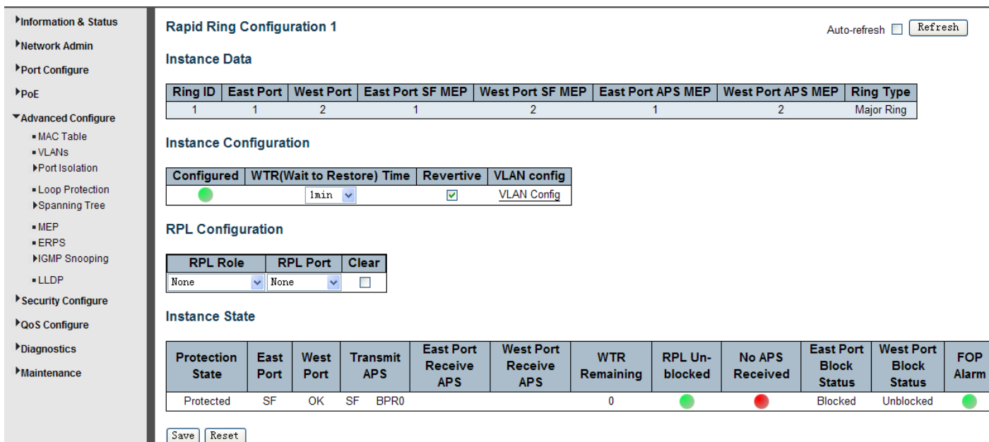
Figure 5-9 EPRS Ring Configuration
