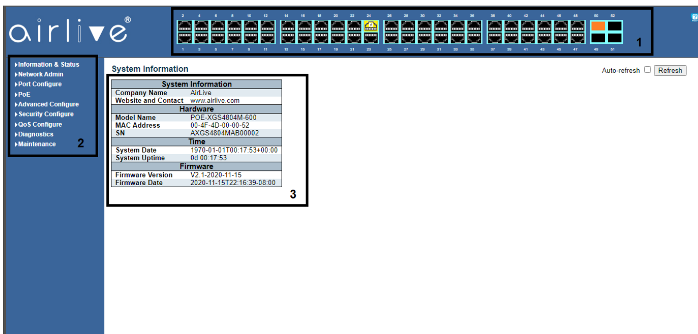
Figure1-2 Web management Main Page interface
